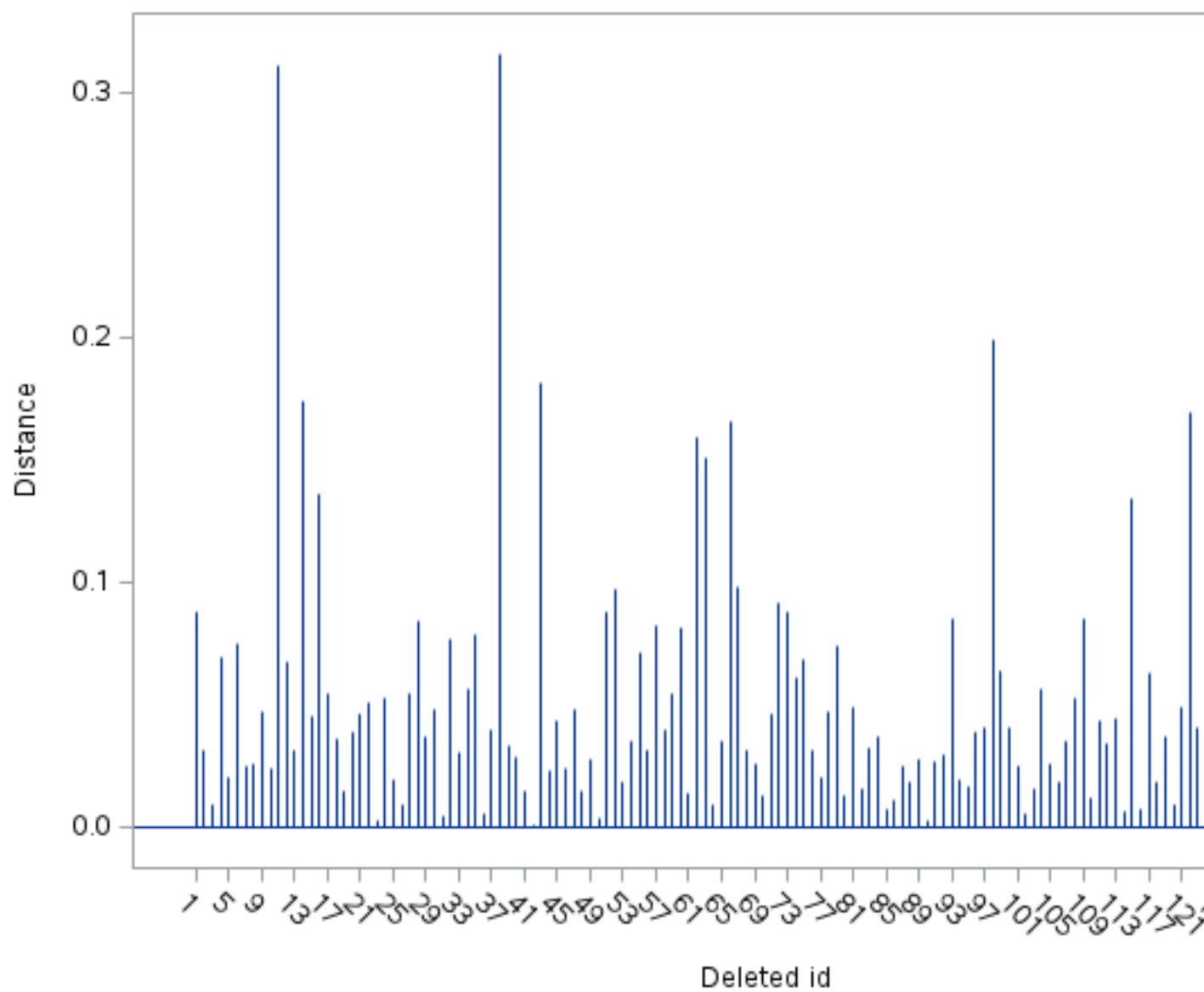
Restricted Likelihood Distance
